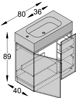
Left version Version gauche SX Version links
